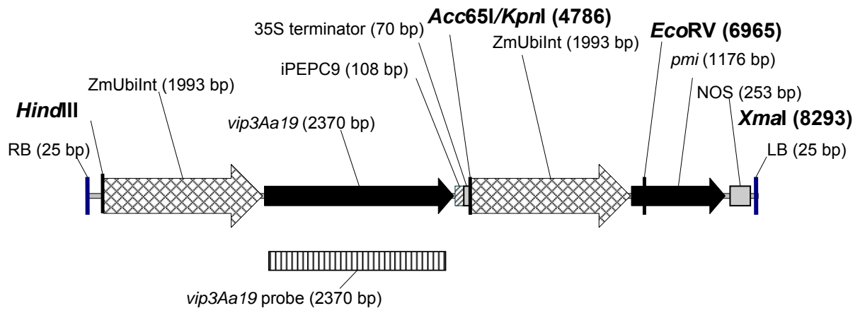
Figure 1: Genes and regulatory elements inserted in MIR162
